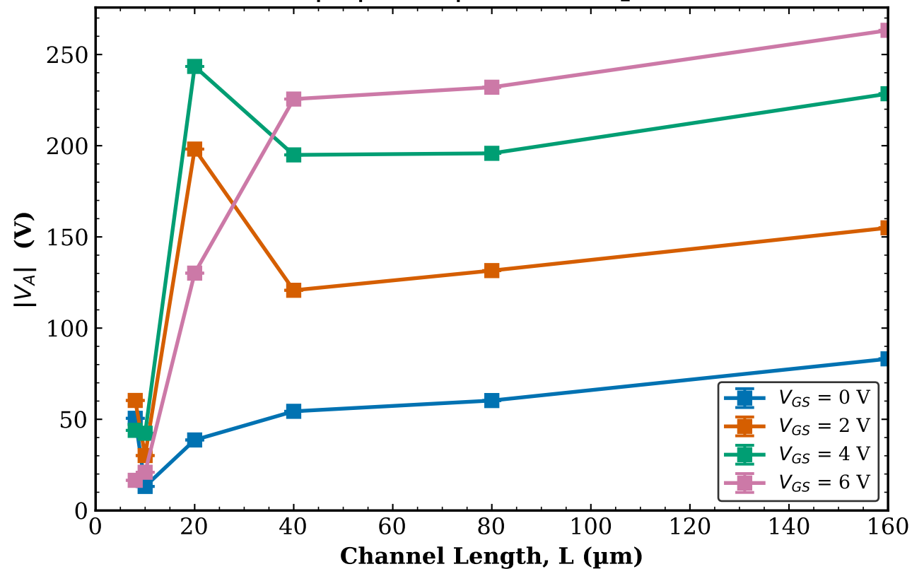
TFT1 Transistor 2 |V_A| vs L | W = 100\text{ }\mu\text{m}
